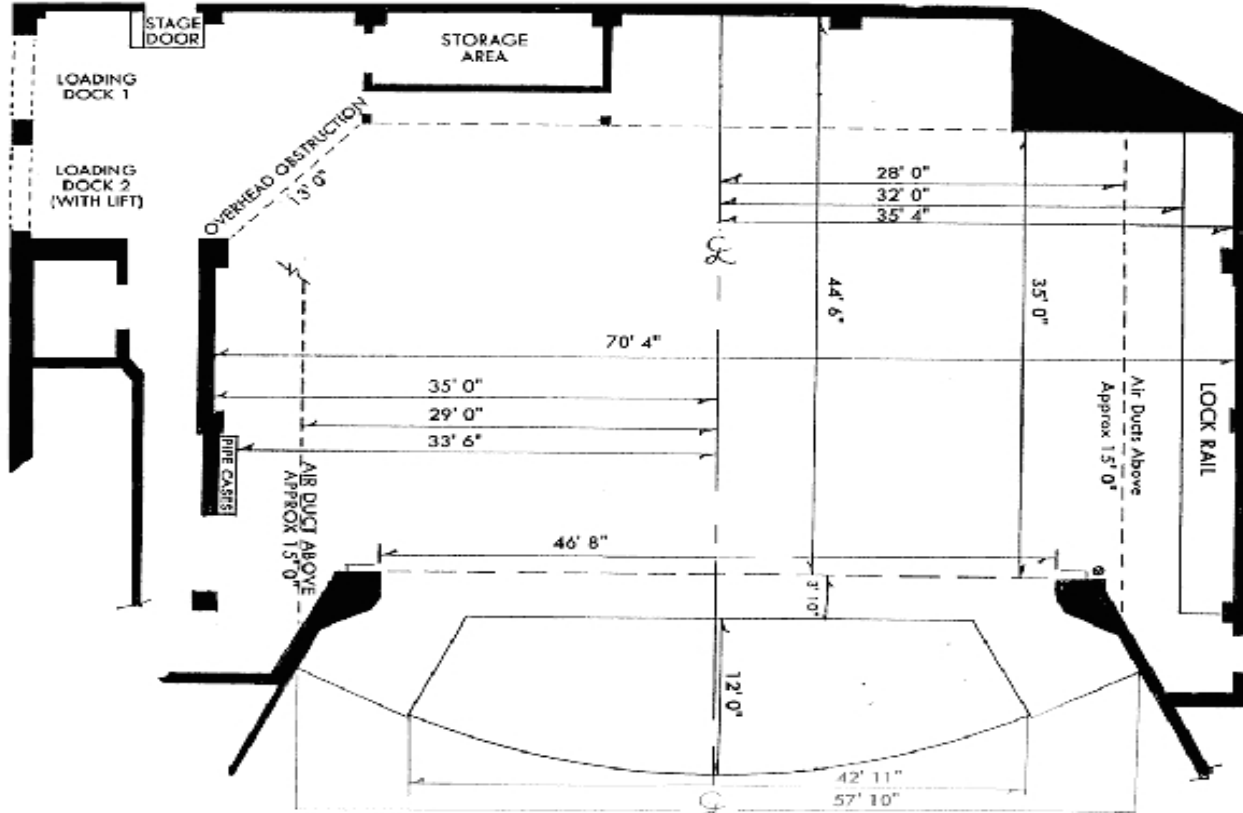
COMMUNITY ARTS CENTER NOT TO SCALE
